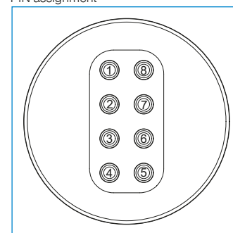
PIN assignment
