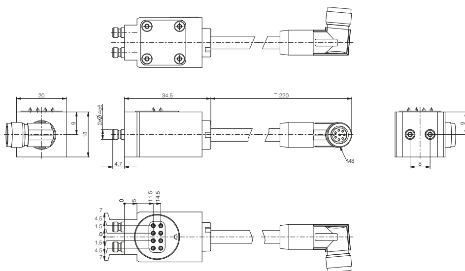
PIN assignment
